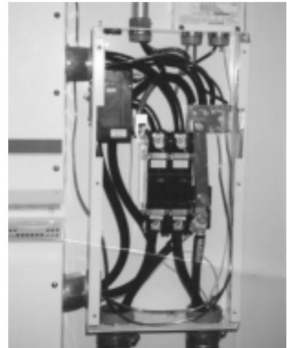
DC circuit breaker box (cover removed) showing much larger components and wire required to protect inverter (on left) and charge controller (on top)
